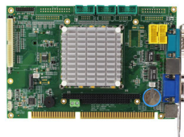
VDX2-6524-CF (Front)
